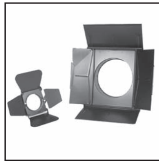
BD Barndoor 4-way adjustable blades used to control beam definition and excess light spill.
