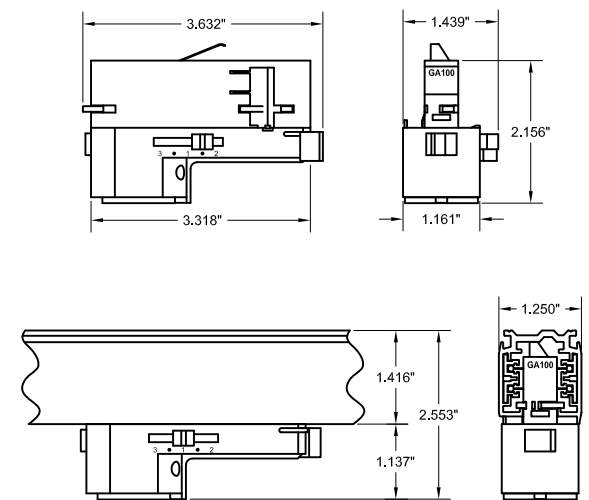
TA3 Specification Grade 120V, 3 circuit Track Adapter.
