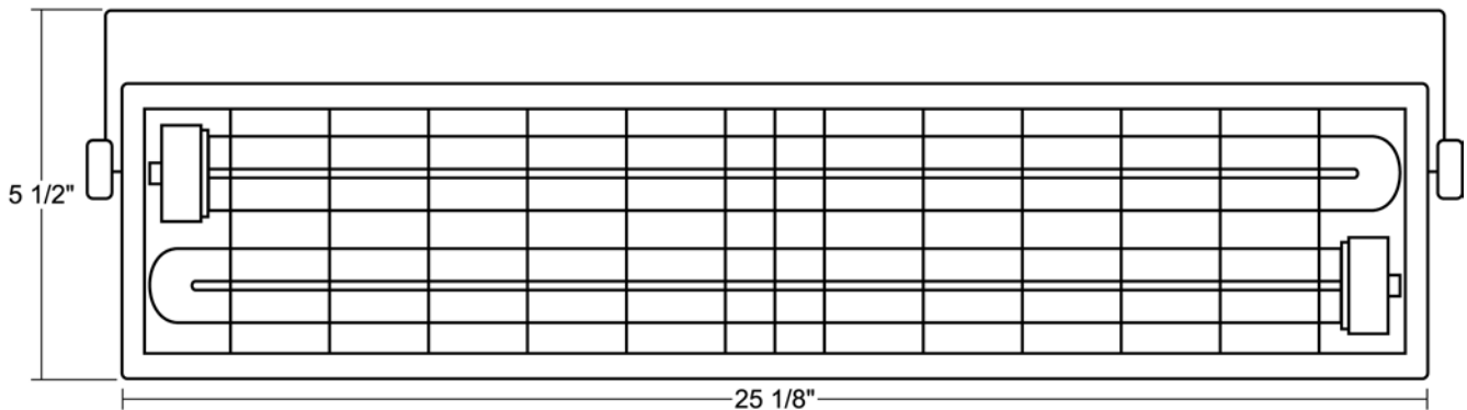
FF40: Front View (4 1/2" deep)
