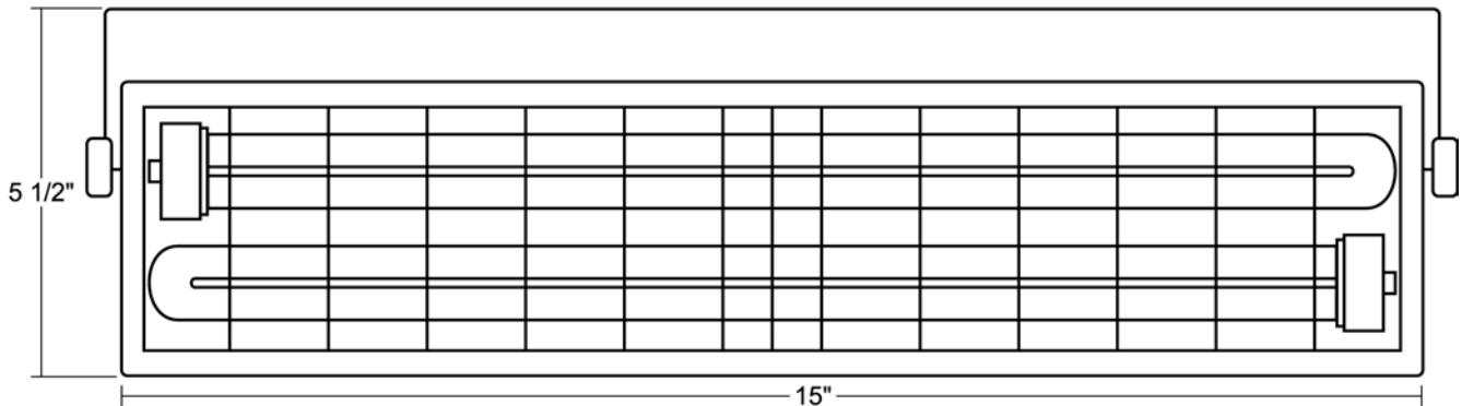
FF18: Front View (4 1/2" deep)
