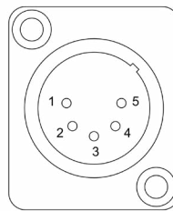
XLR 5MALE
