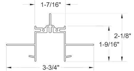
FTPX Flangeless Track Sleeve
