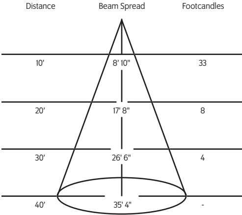
48° Medium Flood Reflector
