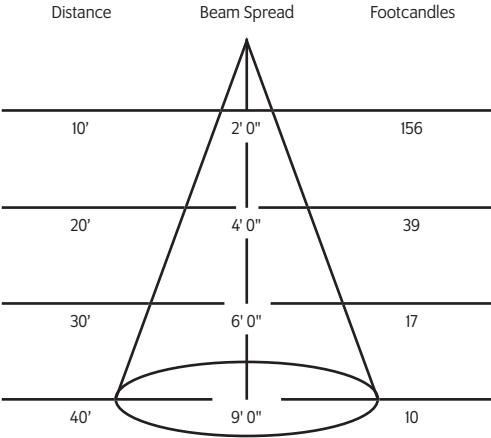
12° Spot Reflector
