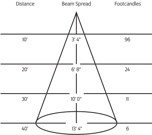
19° Medium Flood Reflector
