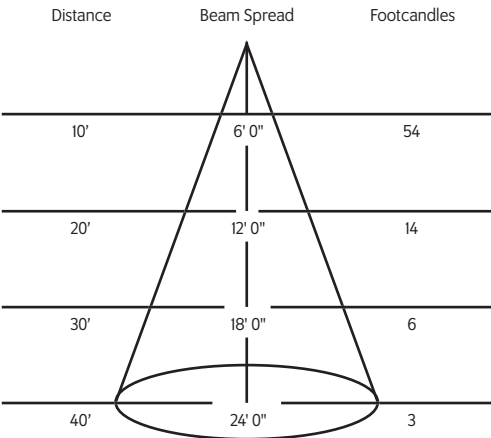
33° Flood Reflector
