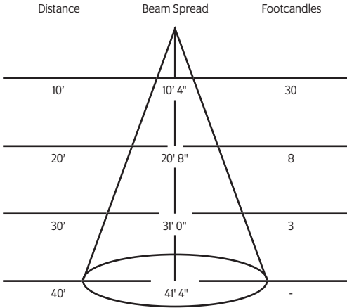
55° Medium Flood Reflector
